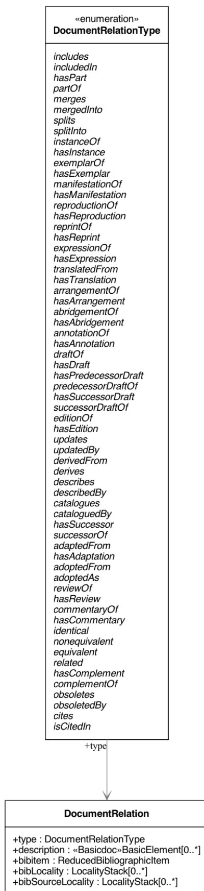
Figure 23 — DocumentRelation and related models
